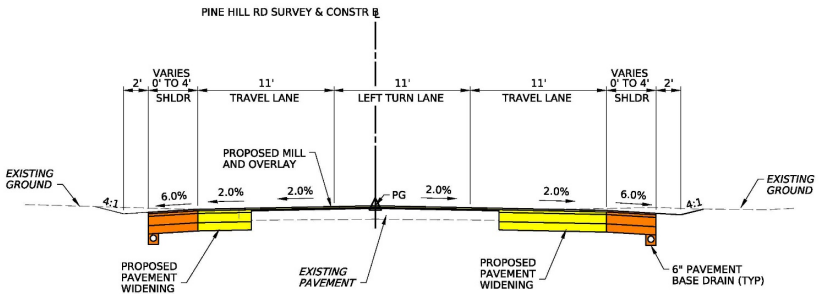
PINE HILL RD ADDED LANE SECTION NOT TO SCALE
