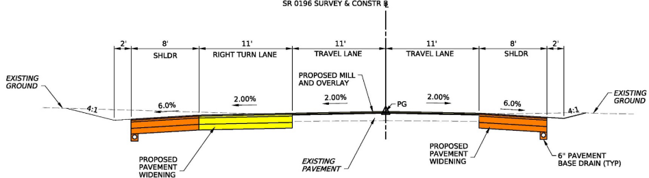
SR 0196 ADDED LANE SECTION NOT TO SCALE
