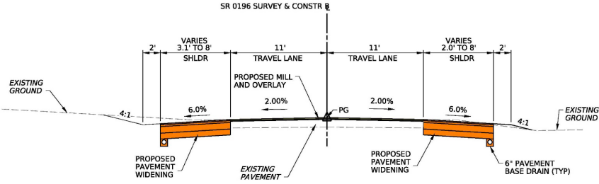
SR 0196 ROADWAY SECTION NOT TO SCALE
