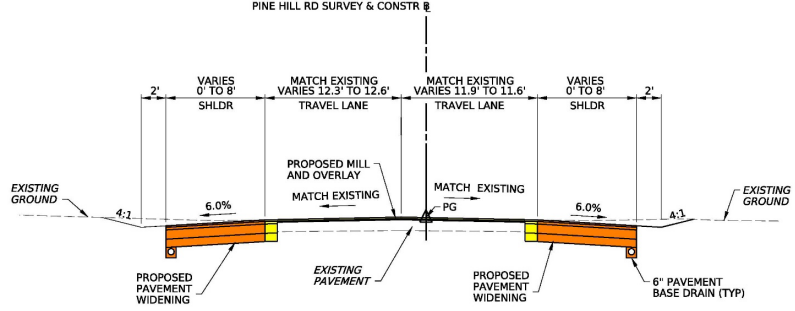
PINE HILL RD ROADWAY SECTION NOT TO SCALE
